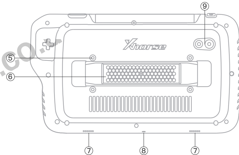
Fig. 4.2.2 Back View
